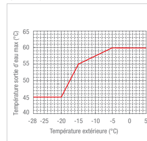
PUZ-HWM140VHA
